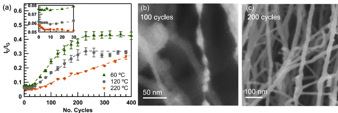
Fig. 2. (a) The difference in the intensity ratio between the D- and G-bands ( I_D/I_G ) of the SWCNTs coated with \text{TiO}_2 at different temperatures as a function of the number of cycles. SEM images of (b) 100 cycles and (c) 200 cycles of \text{TiO}_2 deposited at 60^\circ\text{C} .
