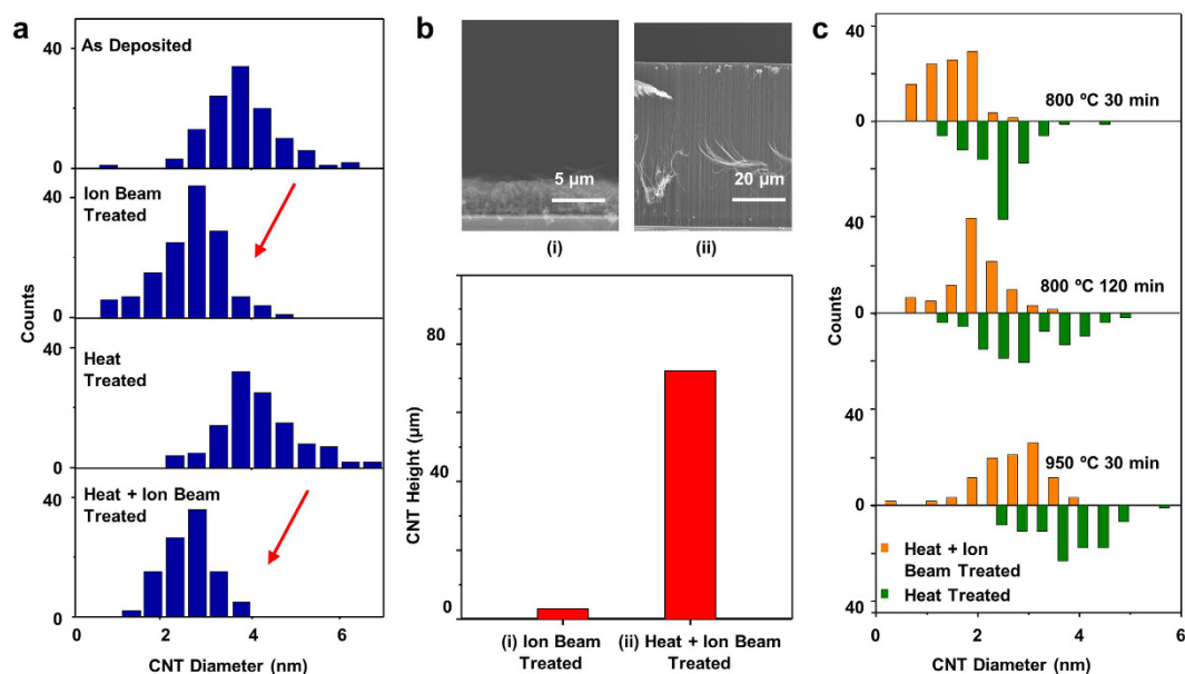
Figure 2. Impact of alumina treatments on CNT diameter and height. CNTs are grown by identical Fe catalyst of 2 Å under same CVD condition on different alumina supports. The diameter distribution of CNTs characterized by TEM images are shown in (a). Ion beam treatment applied on alumina substrate results in a reduction of CNT diameter, as shown by the red arrows in (a); heat treatment applied on alumina leads to slight increase of CNT diameter. The height of CNTs after 5 min of growth on two alumina samples, ion beam treated (4 μm) and heat plus ion beam treated alumina (77 μm), are characterized by SEM images and are compared (b). The impact of heat treatment condition on diameter of CNTs is illustrated in (c), by comparing the diameter distribution of CNTs grown on heat + ion beam treated (orange) and heat treated alumina (green). Three heat treatment conditions are applied to alumina: 800 °C 30 min, 800 °C 120 min, and 950 °C 30 min.
