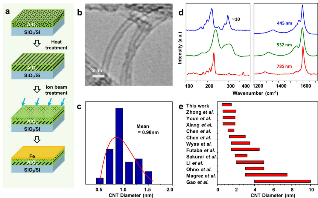
Figure 1. Sequential treatments of alumina and the as-grown sub-1.5-nm VA-CNTs. (a) E-beam deposited alumina is brought to and kept at high temperature of 800 °C for 30 min and then bombarded by Ar + beam of 600 eV for 1 min before 1-Å-thick (nominal thickness) Fe catalyst is deposited. (b,c) The transmission electron microscope image (scale bar: 2 nm) and the histogram of the as-grown nanotubes show an average mean diameter of 0.98 nm and upper bound of 1.5 nm. The nanotubes are single walled. (d) Raman spectra of the as-grown VA-CNTs for the excitation wavelengths of 785 nm (red), 532 nm (green), and 445 nm (blue). (e) Diameter distribution of VA-CNTs obtained by the present and previous reports 10,17,18,25,26,28,32,35–37,51,52 .
